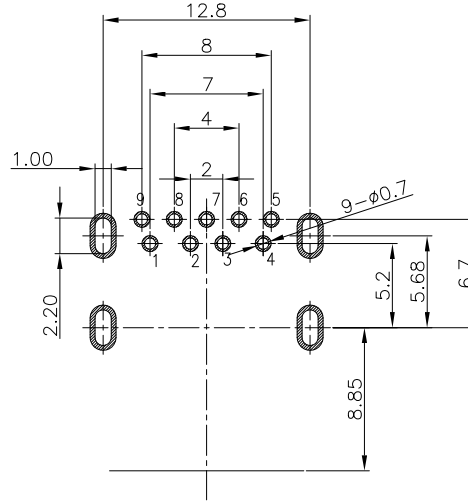
PCB LAYOUT(TOP VIEW T=1.60)
